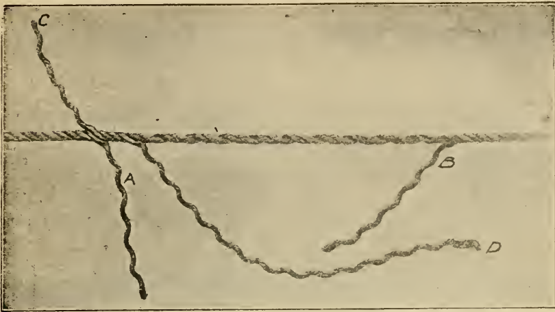
Fig. 4. In Laying In the New Strand the Original Twist and Tension Must Be Maintained
